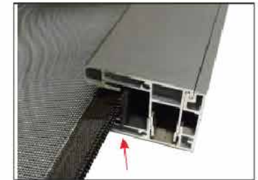
Zipper Track Zipper track system on both side of fabric for better pressure endurance.
