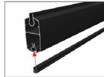
Bottom Seal Anti-collision seal installation at the lower part of blind to protect fabric and blind.
